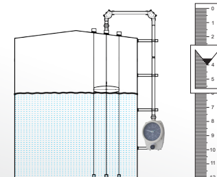
Tank Level Indicator
